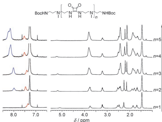
Figure 1. Top: General structure of the oligosquaramides ( n=1-5 for 1–5 , respectively; Boc = tert -butoxycarbonyl). Bottom: Partial 1 H NMR (300 MHz) spectra of 1–5 in CDCl 3 .
