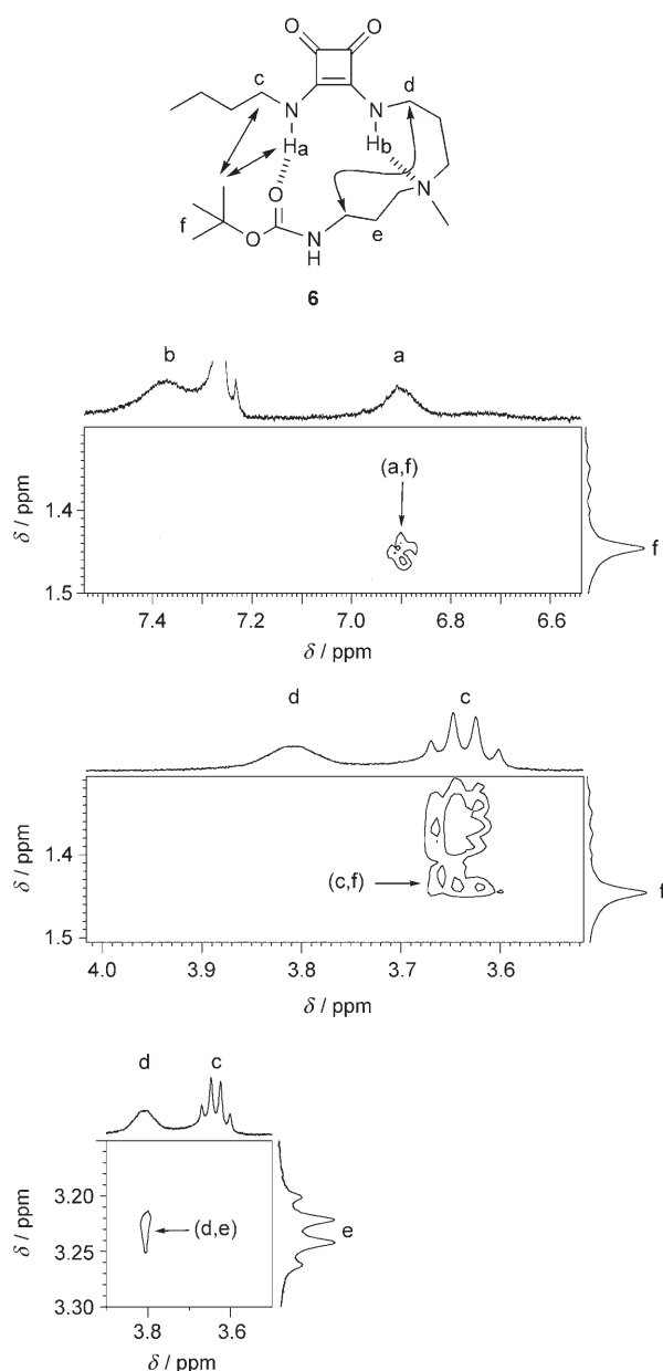
Figure 3. Top: Folded conformation of 6 showing H atom labels and the corresponding NOE interactions. Bottom: NOE interactions as revealed by the NOESY spectrum of 6 in \text{CDCl}_3 .
