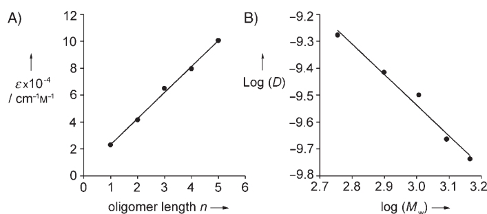
Figure 2. A) The molar extinction coefficients ( \epsilon at 292 nm) in CHCl 3 versus oligomer length ( n ). B) Logarithmic plot of the diffusion coefficient ( D ) versus the molecular weight ( M_w ) of the oligomer.
