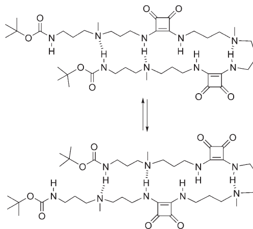
Figure 4. Proposed folded structure for 2 and the slipping equilibrium end-to-end of the hydrogen-bonding pattern.
