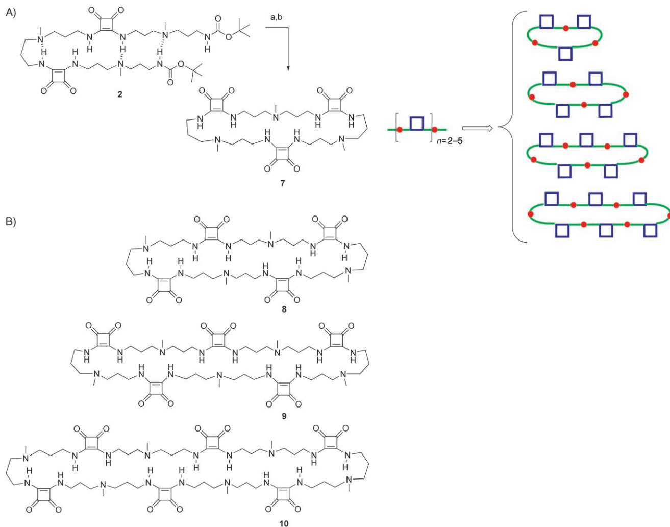
Figure 6. A) Synthesis of macrocycle 7 : a) HCl, 50°C, 3 h; b) diethyl squarate, MeOH, room temperature, 12 h. B) Structures of macrocycles 8–10 .
